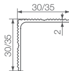
WPC aluminium finishing strip „L" shape dimension (mm)
