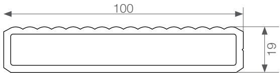
Universal WPC profile/vertical fence panel
