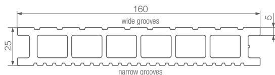
board dimensions (mm)
