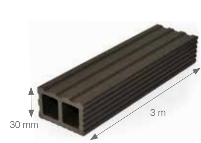
WPC joist
